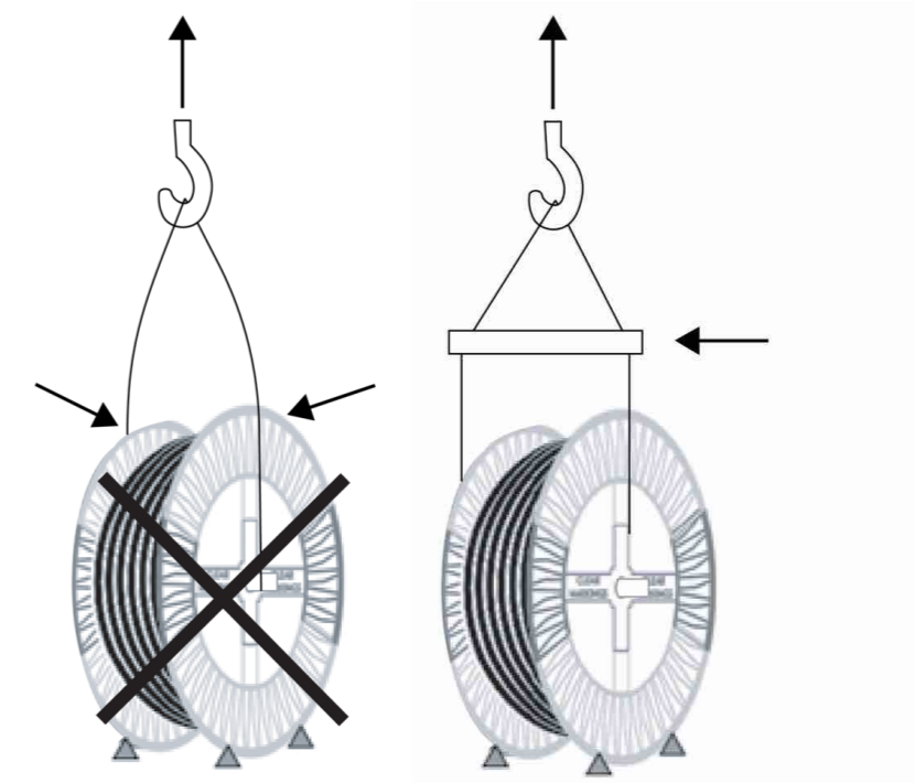
Lift the cable drums using crane & support.
