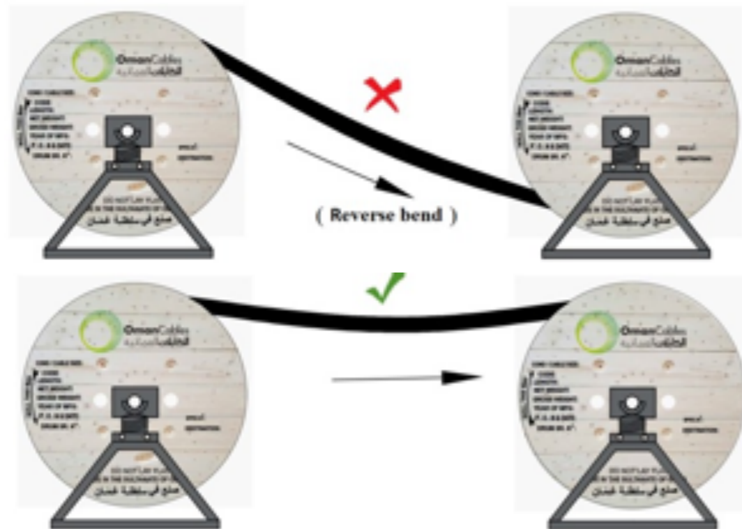
Cable drum re-winding shall be done as shown in above figure.
