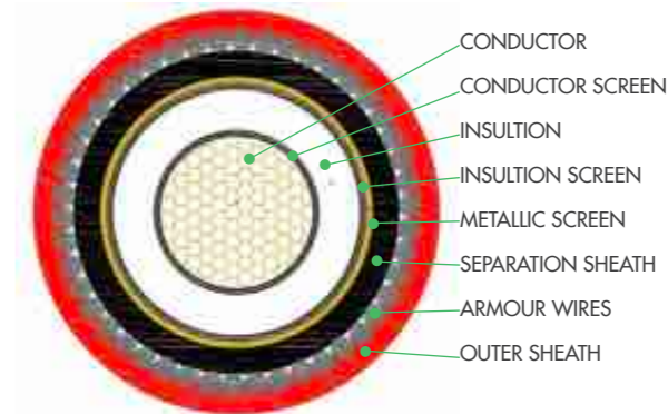
Typical Cross-sectional Diagram Of Single Core Armored Medium Voltage Cable
