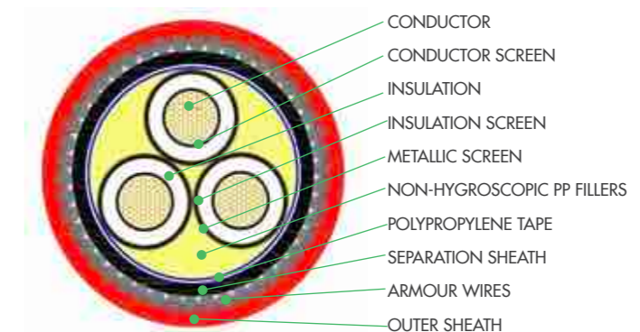
Typical Cross-sectional Diagram Of Three Core Armored Medium Voltage Cable
