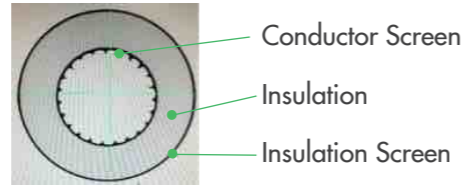
Typical Cross-sectional Diagram of Triple Extrusion MV Layer
